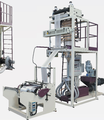
HDPE/LDPE blown film machine
