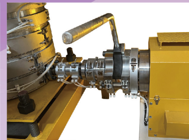
Lever type manual screen changer
